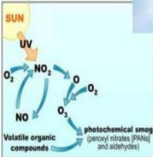
FORMATION OF PHOTOCHEMICAL SMOG
